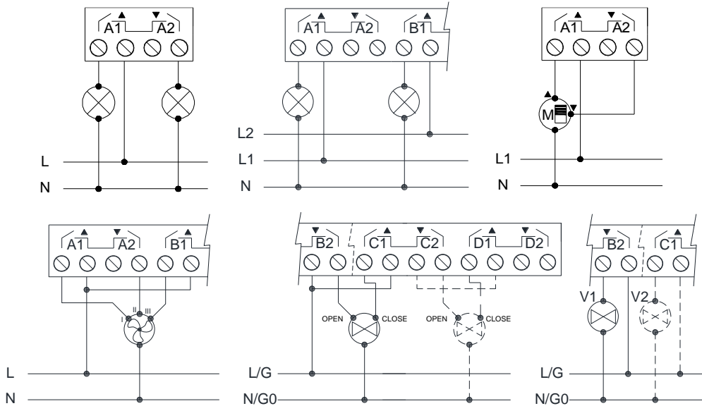
Figure 1: Wiring example (from top to bottom and left to right): 2 loads, 2 loads connected to different phases, shutter channel, fan coil three-speed fan, fan coil three-point valves and fan coil open/close valves.
