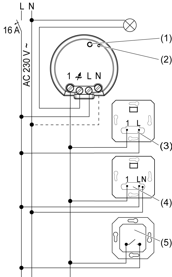
Figure 1: Connection diagram
