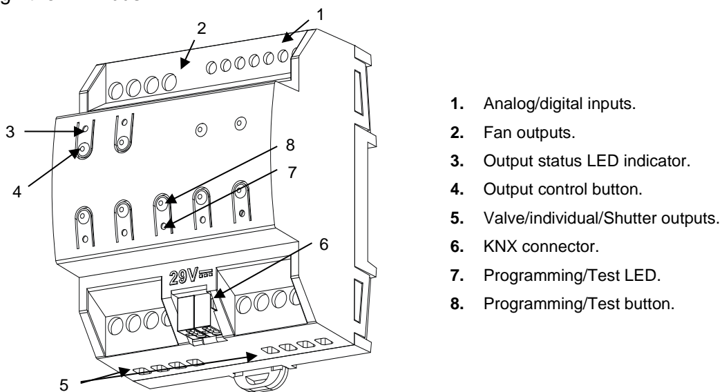
Figure 1 MAXinBOX Hospitality v2 Elements.
