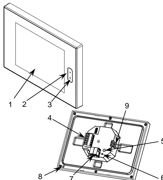
Figure 1. Schematic diagram Z35.
