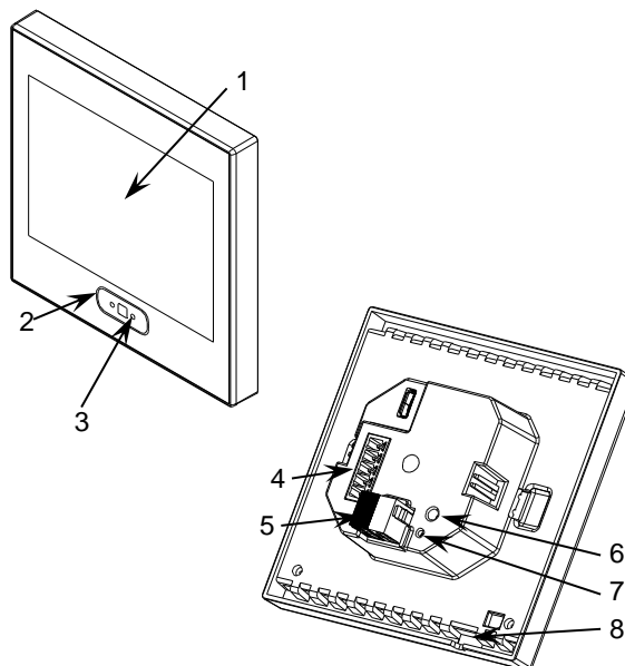
Figure 1. Schematic diagram Z35.
